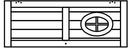
(1) DP2 - SIDE DOOR PANEL - W2A01954 1 1/8"x16 1/2"x43 7/8" (27x420x1126)
