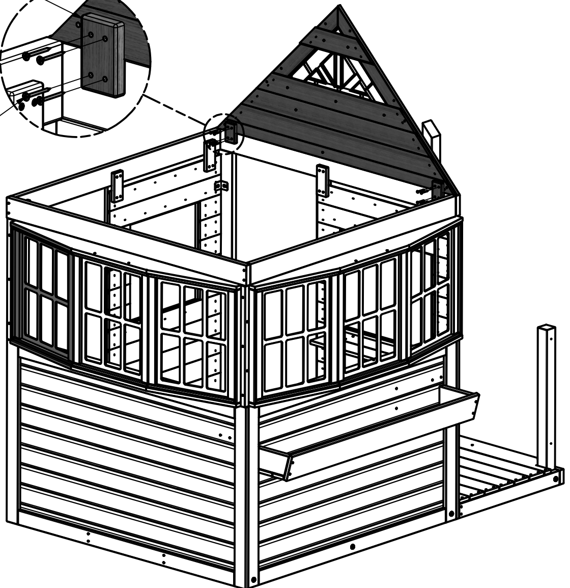
SCREW PFH 8x1 1/2 SD (8 PLCS)
