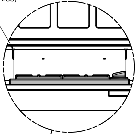
SCREW PFH 8x1 1/8 SD (4 PLCS)
