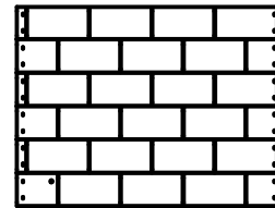
(1) RP4 - RIGHT PORCH ROOF PANEL - W2A01952 1 3/8"x49 1/8"x19 3/8" (35x642x483)
