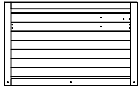
(1) WP3 - LOWER LEFT SIDE PANEL - W2A01945 1 1/4"x49 7/8"x29 3/8" (27x1200x745)
