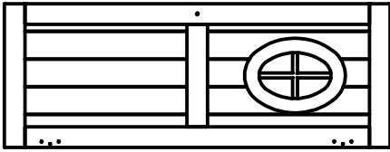
(1) DP1 - FRONT DOOR PANEL - W2A01953 1 1/8"x16 1/2"x43 7/8" (27x420x1126)
