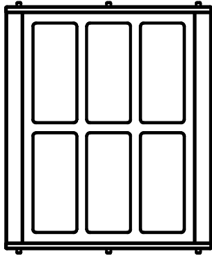
(6) BAY WINDOW PANEL - A100373
