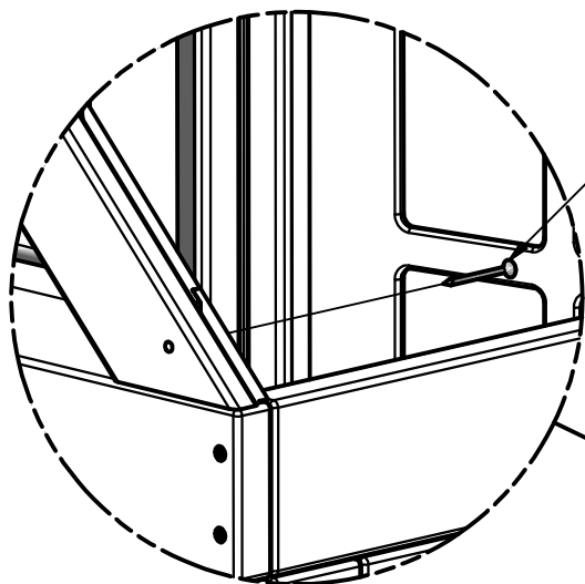
SCREW PFH 8x1 3/4 SD (8 PLCS)
