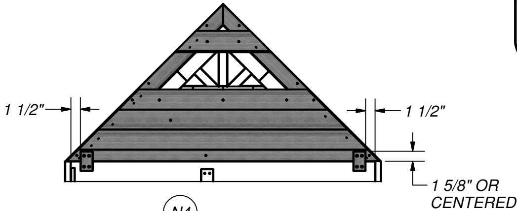
(1) GP1 - FRONT FRONT PANEL - W2A01947 1 1/8"x50"x25" (27x1269x634)
