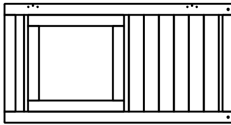
(1) WP1 - FRONT RIGHT SIDE PANEL - W2A01943 1 1/8"x25 3/8"x48 7/8" (27x643x1240)
