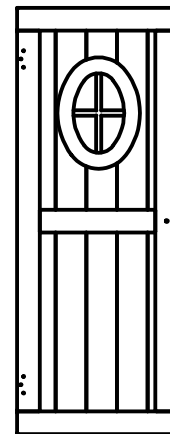
(1) DP2 - SIDE DOOR PANEL - W2A01954 1 1/8"x16 1/2"x43 7/8" (27x426x1126)
