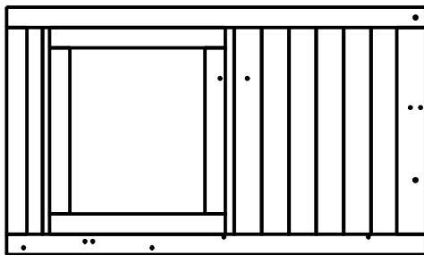
(1) WP4 - FRONT LEFT PANEL - W2A01946 1 1/8"x28 3/4"x48 7/8" (27x730x1240)
