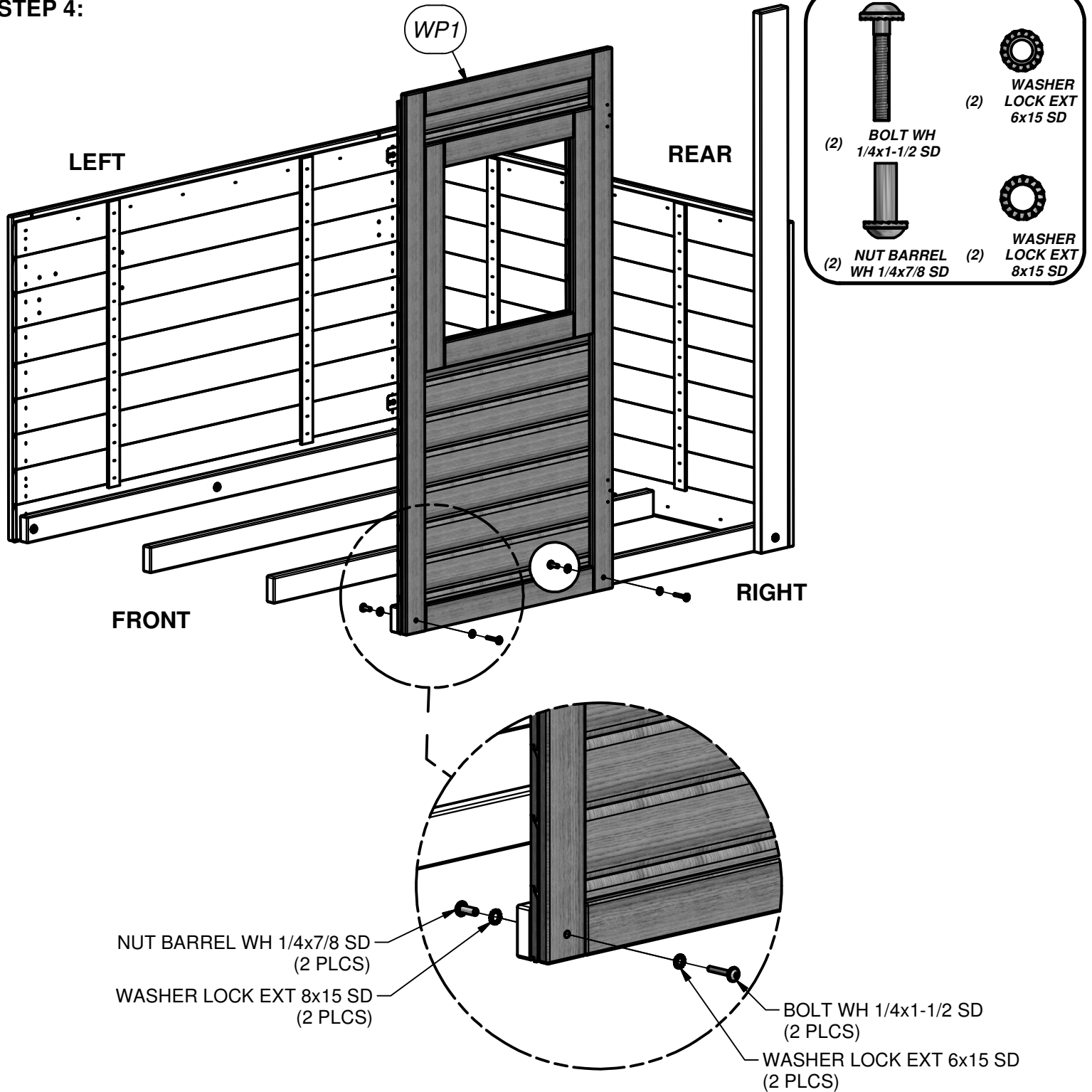
(1) WP1 - FRONT RIGHT SIDE PANEL - W2A01943 1 1/8"x25 3/8"x48 7/8" (27x643x1240)
