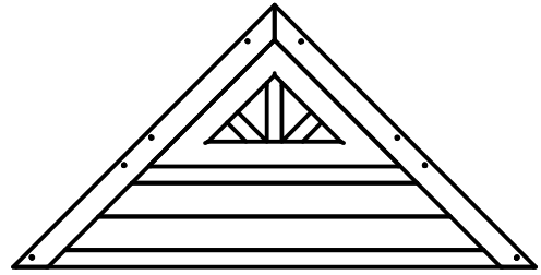
(1) GP2 - REAR GABLE PANEL - W2A01948 1 1/8"x50"x25" (27x1269x634)
