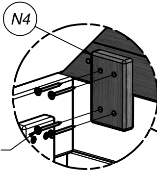
SCREW PFH 8x1 1/2 SD (8 PLCS)
